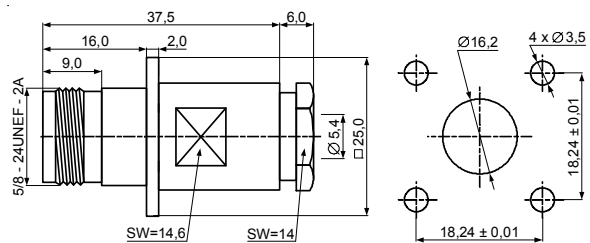
JC3.660.074 N-KF3 SYV-50-3 RG-58/U
