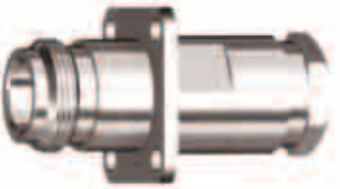
JC3.660.074 N-KF3 SYV-50-3 RG-58/U
