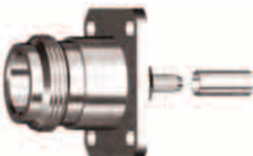
JC3.660.082 N-C-KF1.5 SFF-50-1.5-1 RG-174/U
