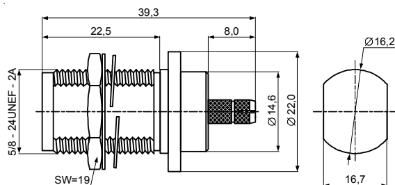
JC3.660.338 N-C-KY3-M SYV-50-3 RG-58/U
