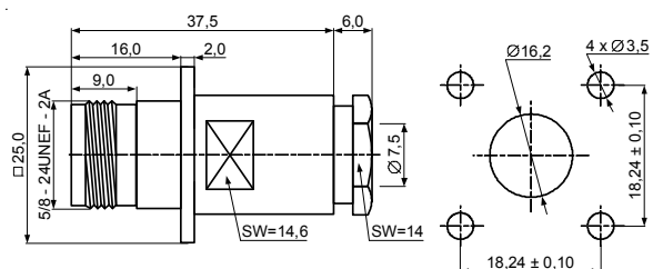
JC3.660.326 N-KF5 SYV-50-5-1
