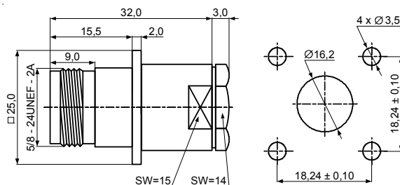
JC3.660.094 N-KFB3-1 SFT-50-3 RG-402/U
