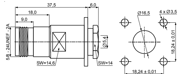
JC3.660.209 N-KF3-1 SYV-50-3 RG-58/U
